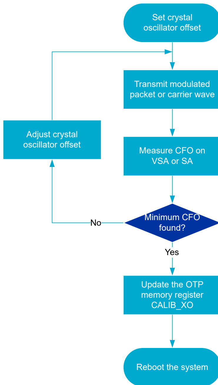
Figure 1: CALIB_XO process for transmit-based approach
