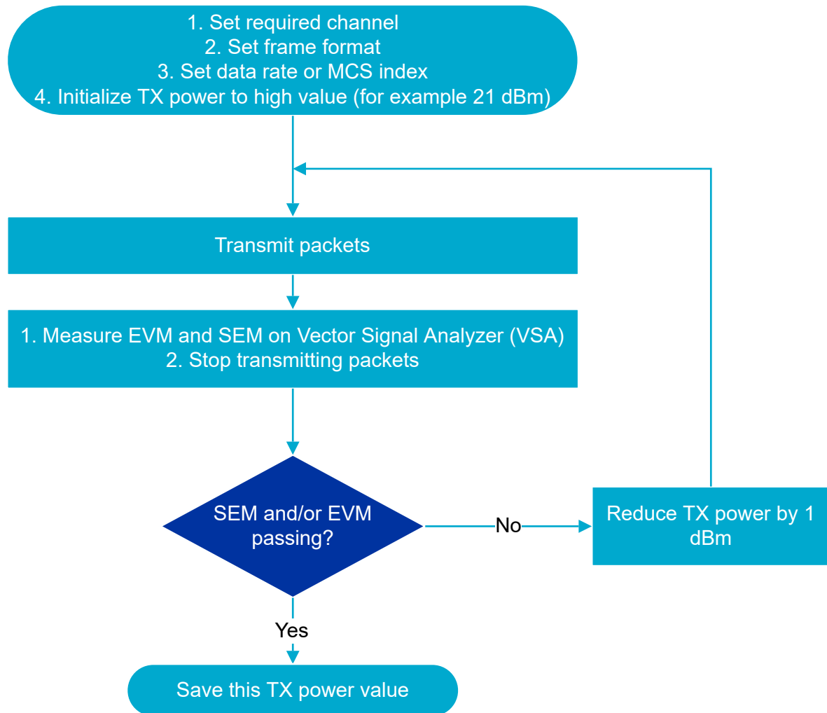
Figure 3: Procedure for determining the maximum TX power
