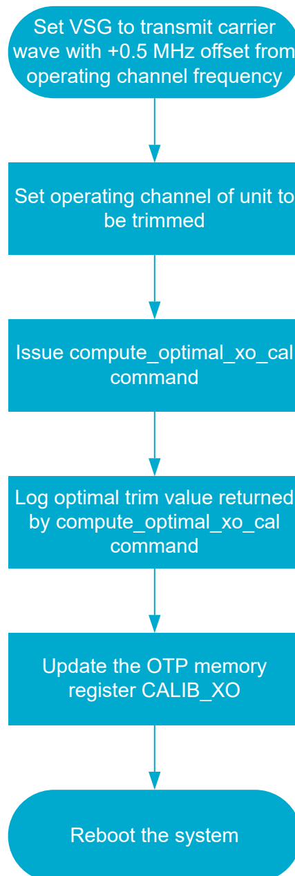
Figure 2: CALIB_XO process for receive-based approach
